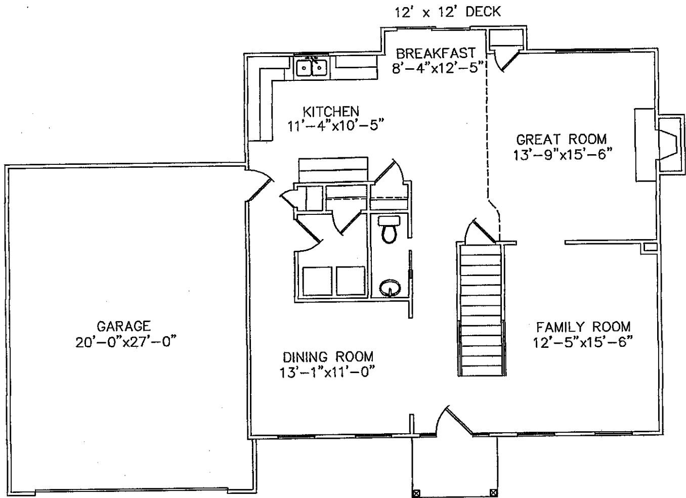
BELLFORD 1st FLOOR PLAN - 1108 SF.
