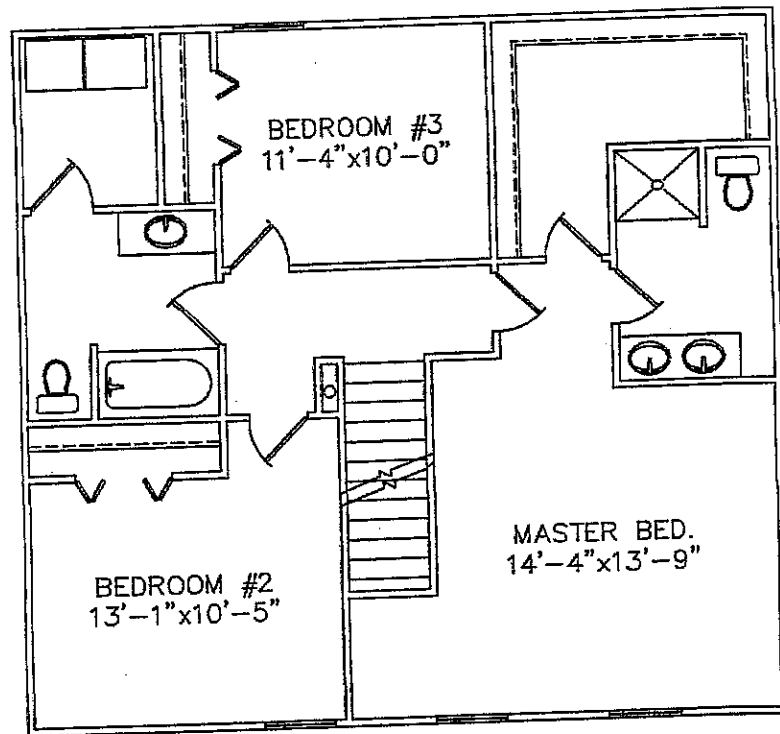
BENNINGTON 1736 STANDARD- 2nd FLOOR PLAN
