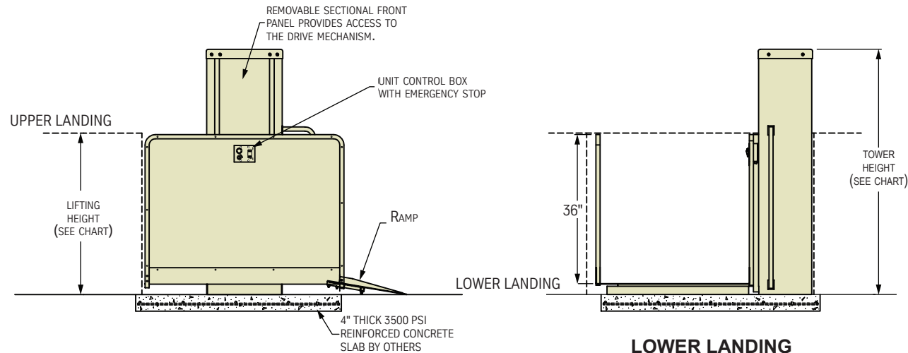
FRONT ELEVATION Right Hand Unit Shown
