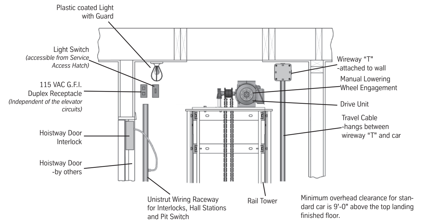
Section thru Top of Hoistway at Drive Unit
