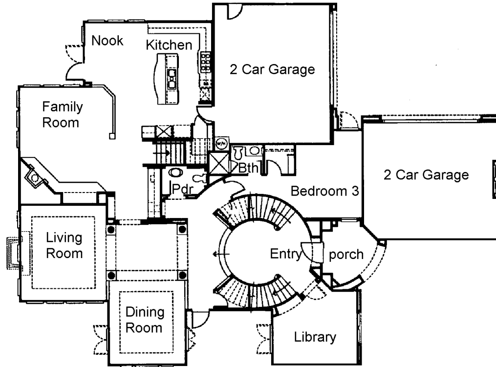
First Floor
