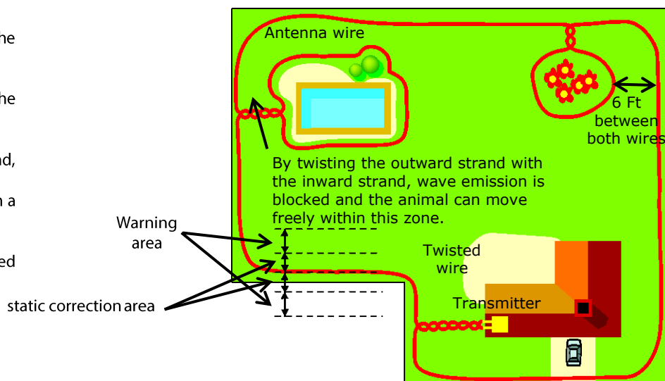
Diagram 4 – Sample installation
